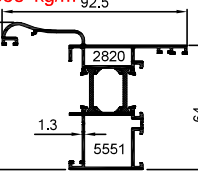
64-2820-5551 1.538 kg/m
