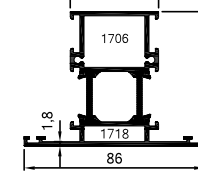
64-3637-3638 1.560 kg/m
