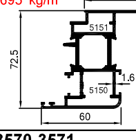
64-3570-3571 2.411 kg/m
