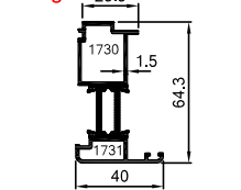
64-3640-3542 2.430 kg/m
