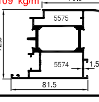
64-5574-5575 2.109 kg/m
