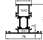
64-5566-5567 1.741 kg/m
