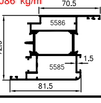
64-5585-5586 2.086 kg/m
